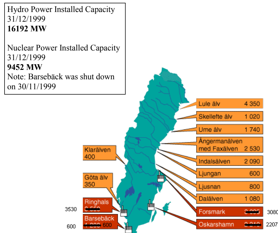
FIG. 2. Location of Power Stations in Sweden
